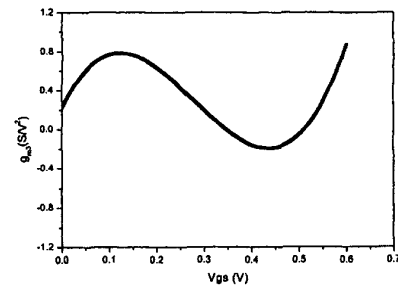
Fig. 3 Simulated gm_3 characteristic of GaAs MESFET using TOM(Triquant Own Model)3 model.
